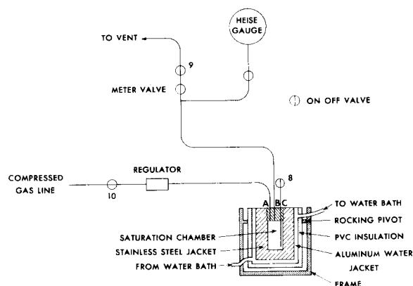
Figure 1. Equilibration system.
