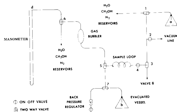
Figure 2. Sampling system.
